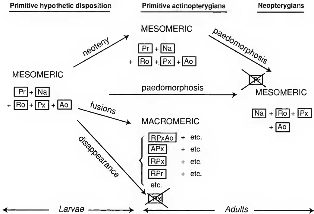
FIG. 4. — Hypothesis proposed in this paper about the evolution of the dermal snout, based on those of Pearson, Schaeffer, Long, Gardiner & Schaeffer (see text). Ao, antorbital; APx, antorbito-premaxillary; Na, nasal; Px, premaxillary; Pr, postrostral; Ro, rostral; RPx, rostro-premaxillary; RPxAo, rostro-premaxillo-antorbital; RPr, rostro-postrostral.
